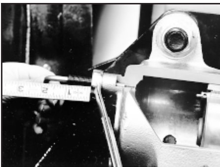
Back out adjusting screw
